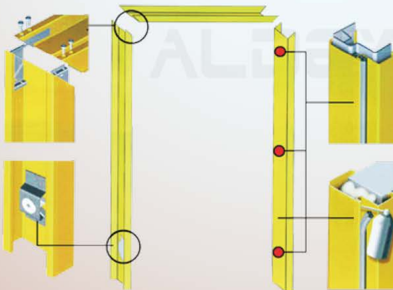
Fire Rated Doors Frame
