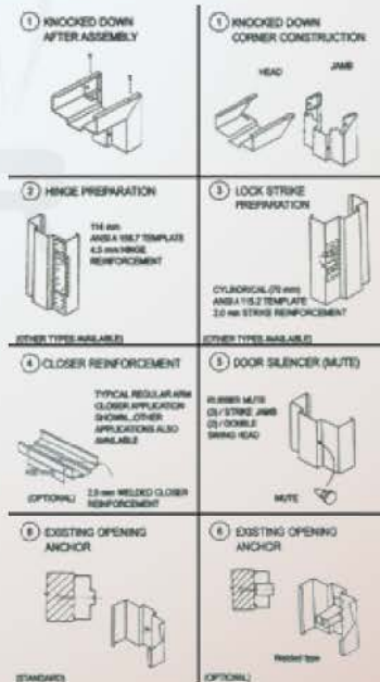
MW Series Frames Construction Features
